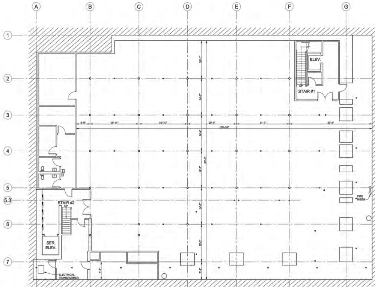
BASEMENT FLOOR PLAN SCALE: 1/8" = 1'-0" AREA = 13,183 SQ.FT.
